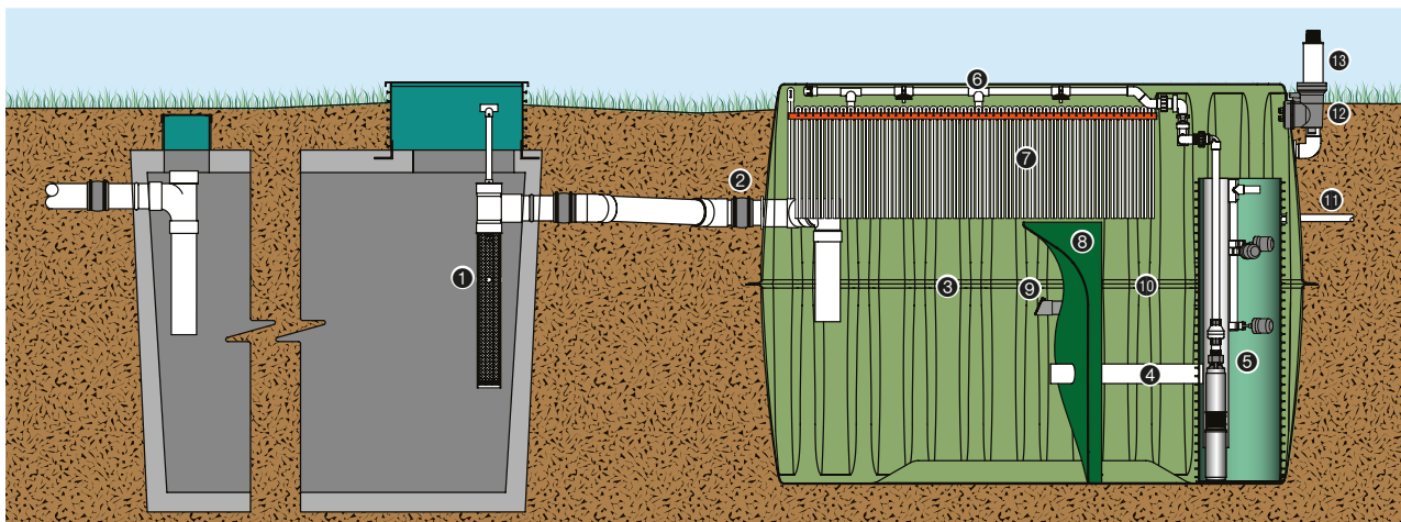
The AX-RT is a completely pre-packaged "plug & play" wastewater treatment system that can be quickly installed right behind an existing (or new) watertight septic tank.
